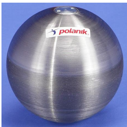
Competition steel unpainted shot put
